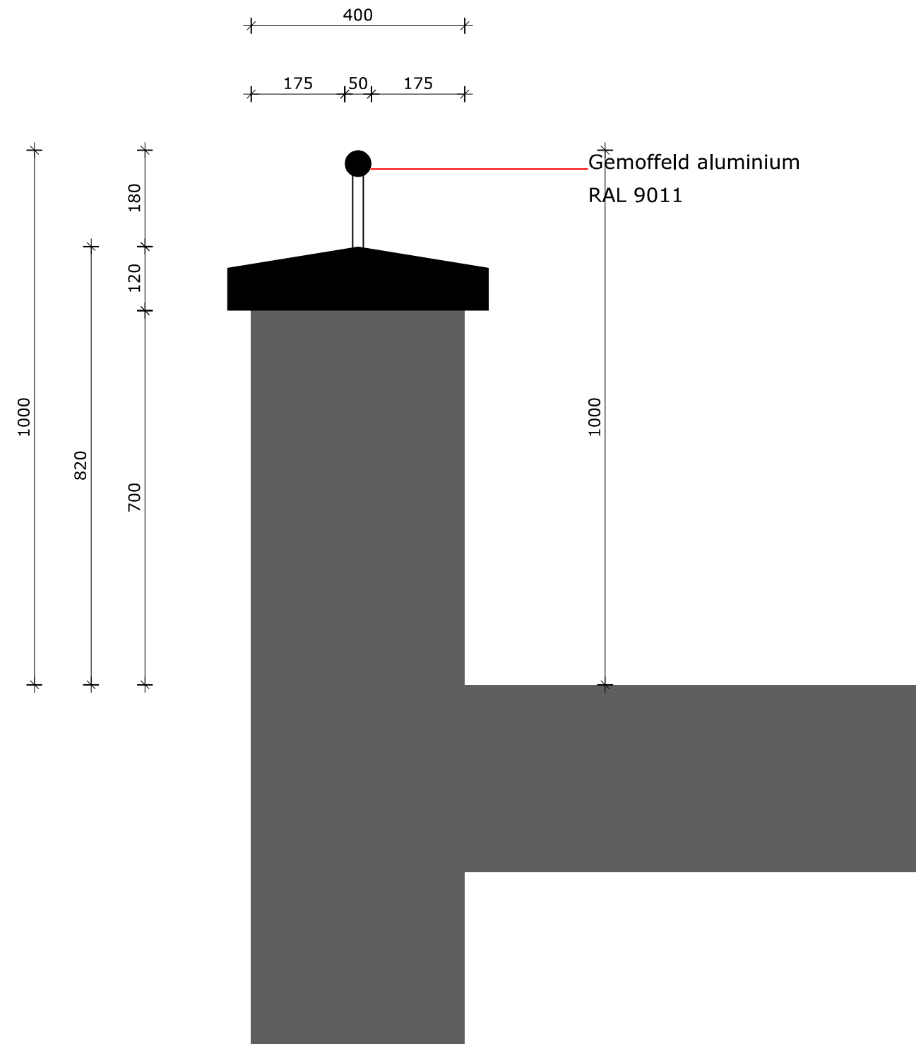
betonafdekker + balustrade C7
